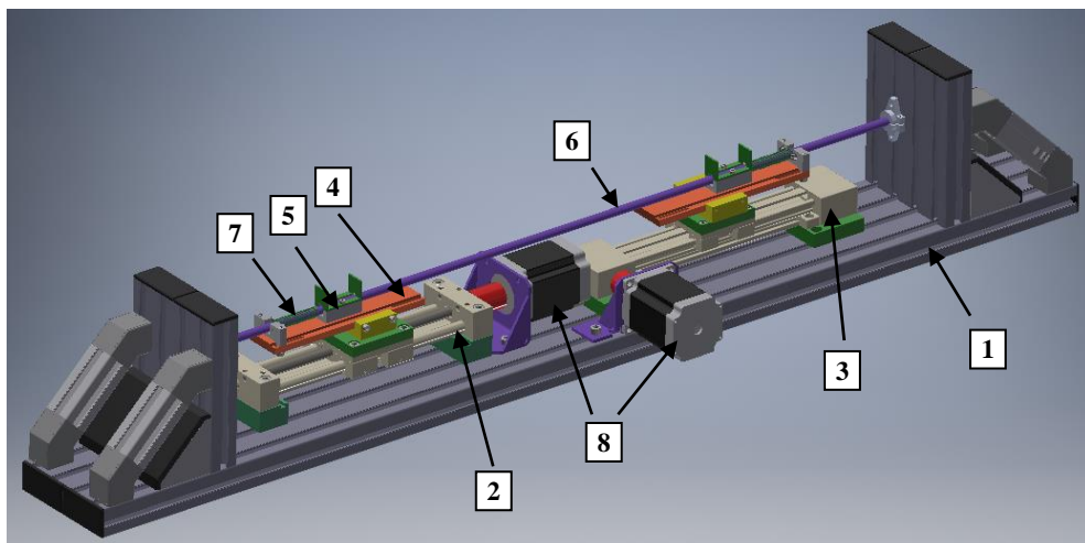
Fig. 1. 3D CAD model of the stand.
